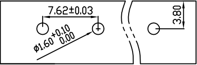
PCB LAYOUT
