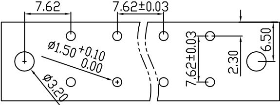
PCB LAYOUT
